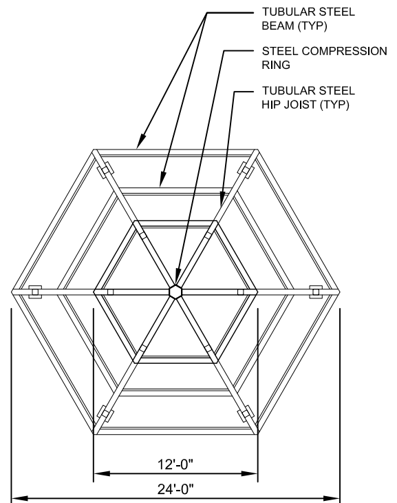
FRAMING PLAN
