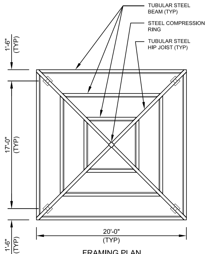
FRAMING PLAN
