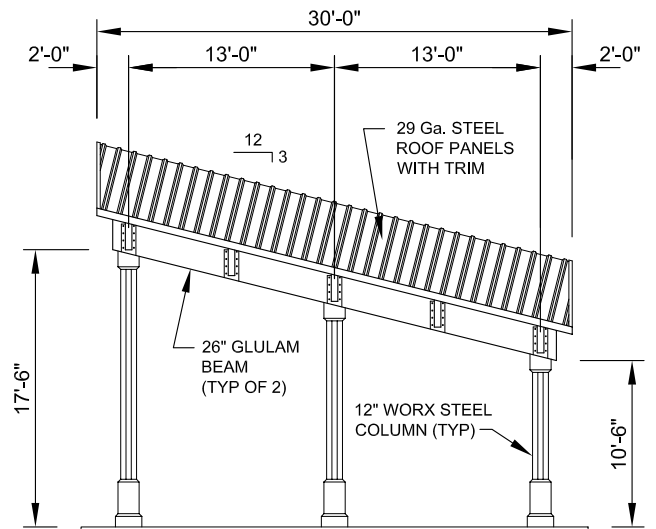
SIDE ELEVATION SCALE: NTS
