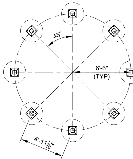
FOOTING LAYOUT PLAN SCALE: NTS
