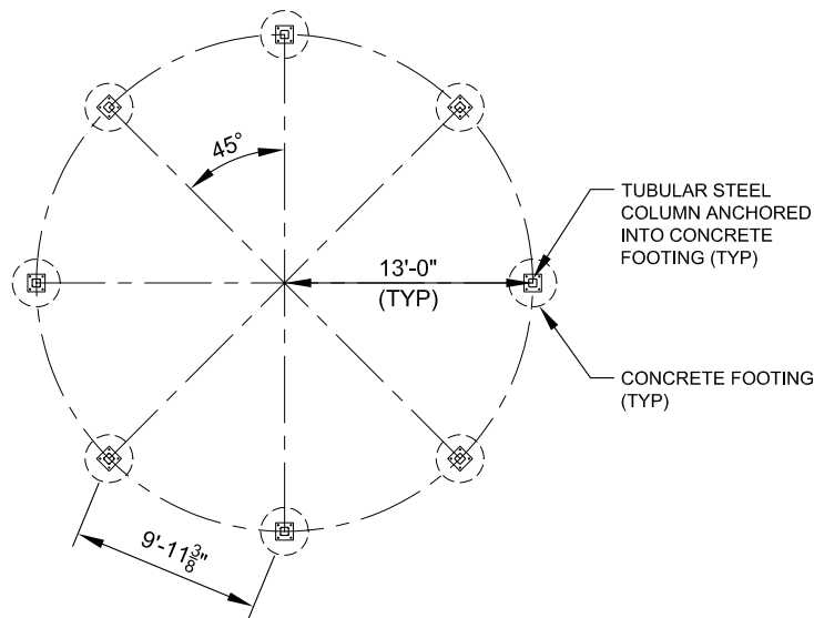
FOOTING LAYOUT SCALE: NTS
