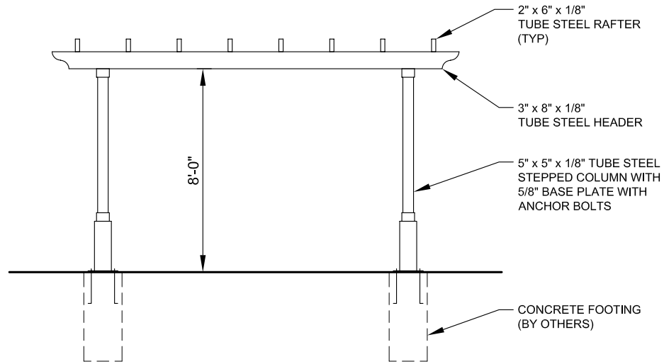
FRONT ELEVATION
