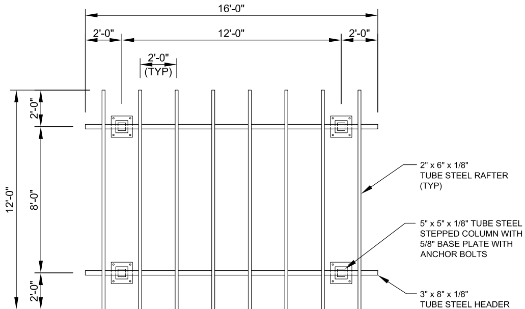
FRAMING PLAN
